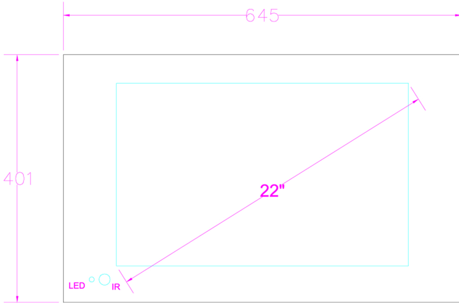
Front Panel
